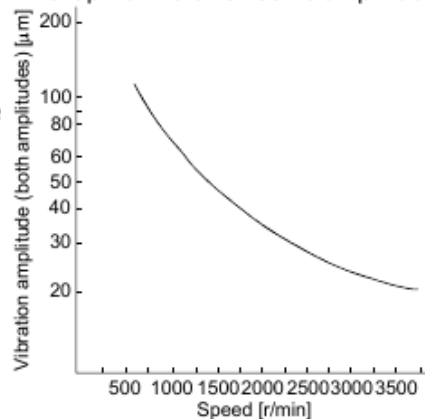
Graph of vibration servo amplitude vs. speed
